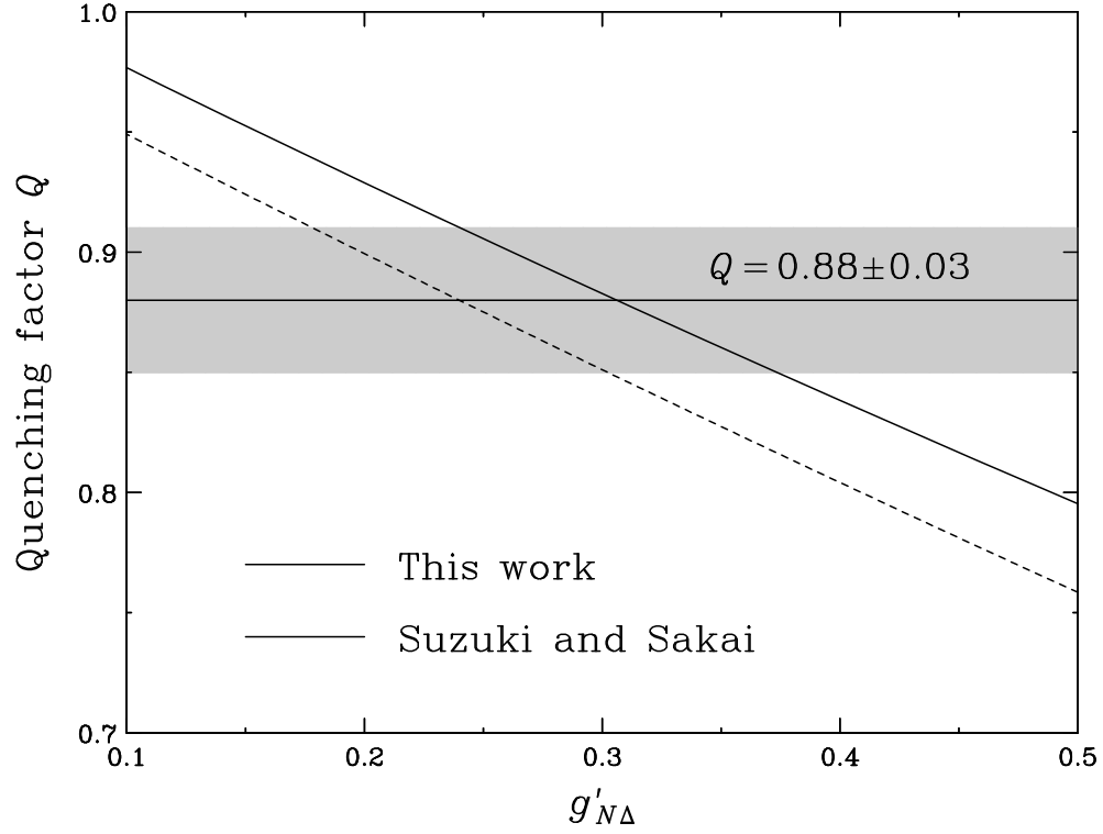
FIG. 3: The GT quenching factor Q as a function of g'_{N\Delta} . The experimental result of 0.88 \pm 0.03 [21] is shown by the horizontal solid line and band. The dashed curve is the theoretical prediction by Suzuki and Sakai [13].
