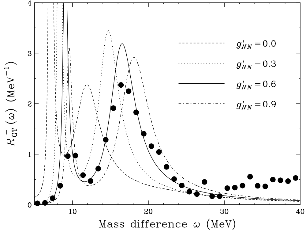
FIG. 1: The g'_{NN} dependence of \text{GT}^- strength distributions from ^{90}\text{Zr} to ^{90}\text{Nb} , where g'_{N\Delta} and m^*(0)/m_N are set to 0.3 and 0.7, respectively. The filled circles are the experimental data taken from Ref. [18].
